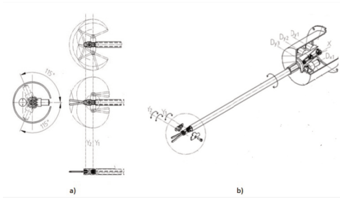
FIGURE 1. Possible instrument workspace and instrument monuments.
